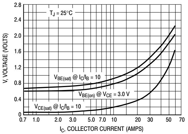
Figure 8. "On" Voltages
